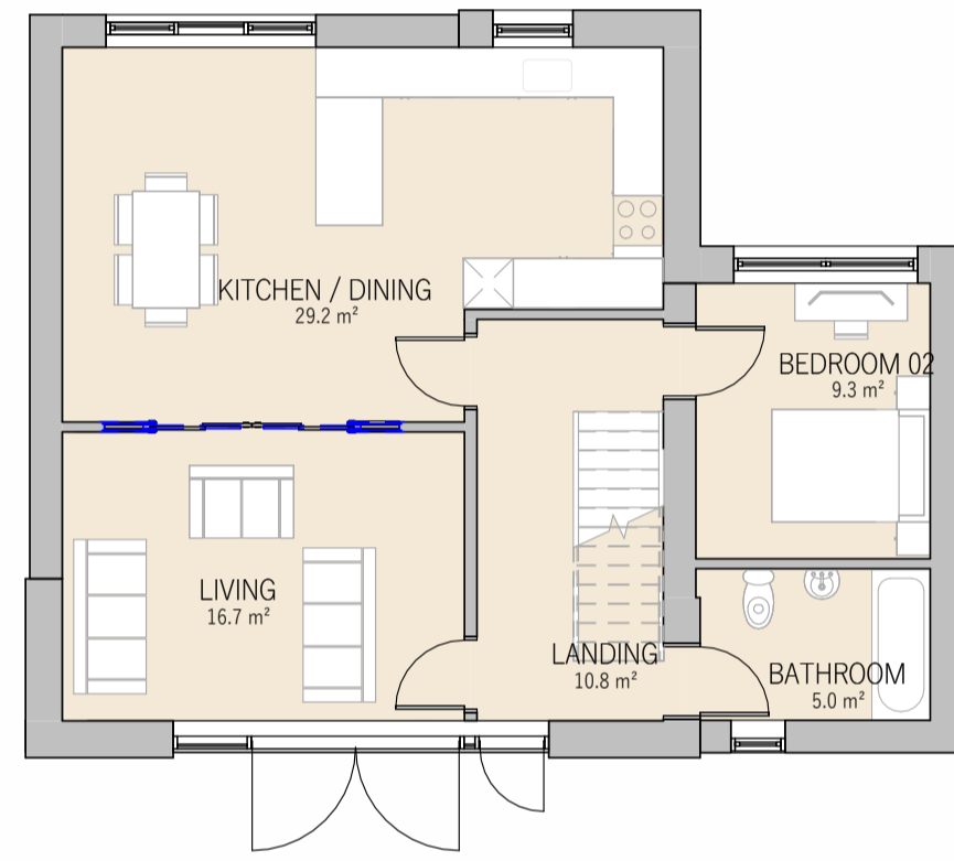
02 - SECOND FLOOR SCALE: 1 : 100
