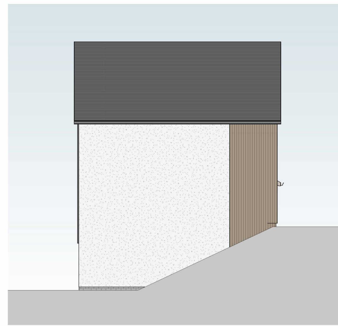
PROPOSED - SIDE ELEVATION SCALE: 1 : 100
