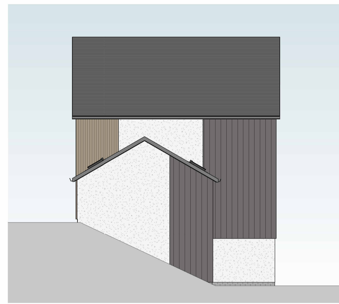
PROPOSED - SIDE ELEVATION SCALE: 1 : 100
