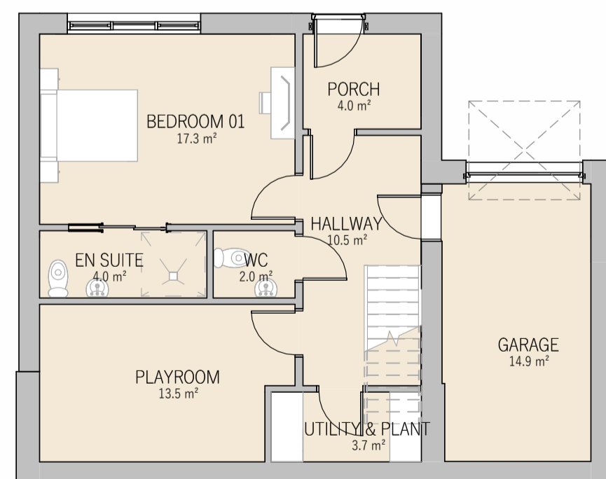
00 - GROUND FLOOR SCALE: 1 : 100
