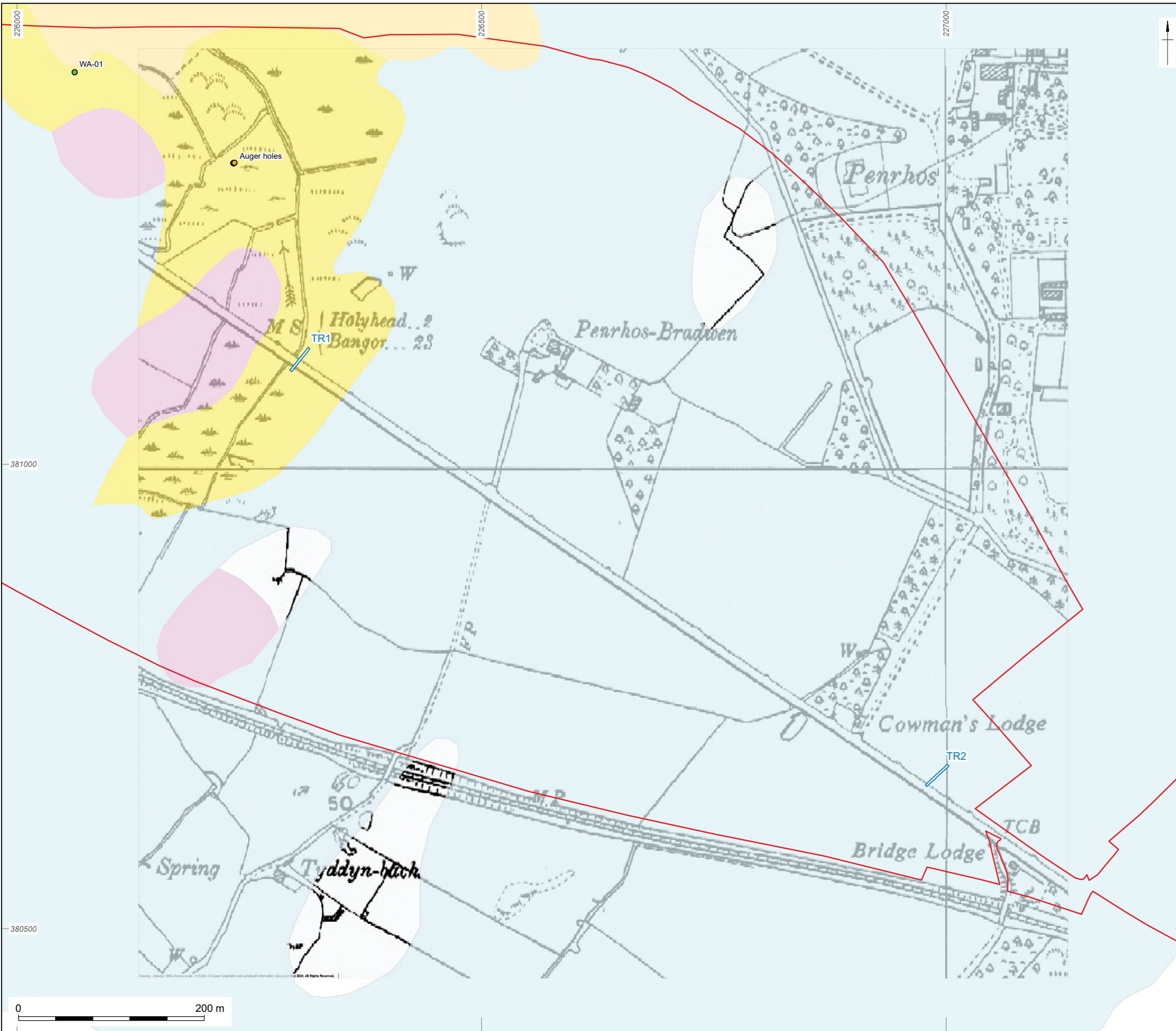
Figure 2: Location of evaluation trenches and geoaerchaeological bore/auger holes against superficial geology and 1963 Ordnance Survey mapping
